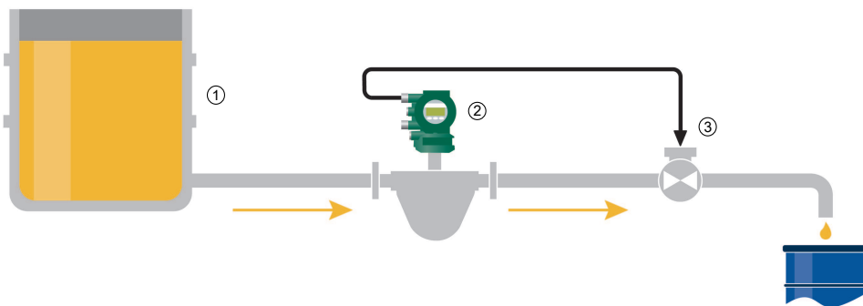
Fig. 41: One-stage mode (The above diagram illustrates the fundamental functionality for one of several combination possibilities)
