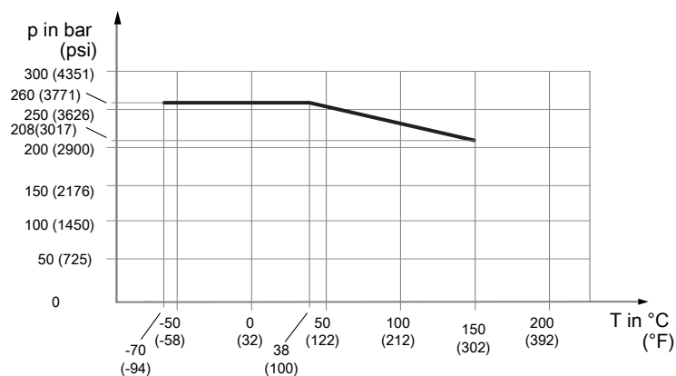
Fig. 15: Allowed process pressure as a function of temperature
