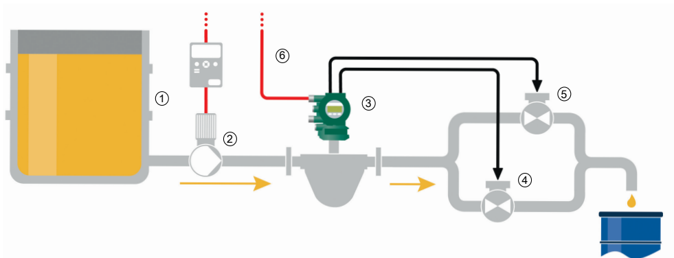
Fig. 42: Two-stage mode (The above diagram illustrates the fundamental functionality for one of several combination possibilities)
