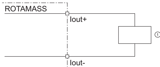
Fig. 22: Active current output connection lout HART
