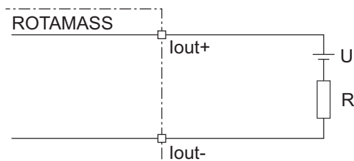
Fig. 24: Passive current output connection I out
