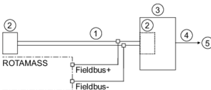
Fig. 38: PROFIBUS PA connection
