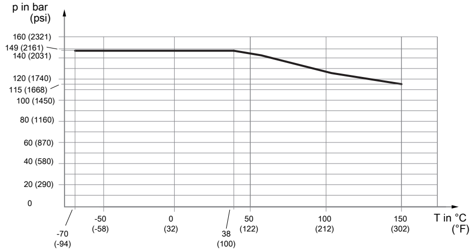
Fig. 13: Allowed process pressure as a function of process connection temperature
