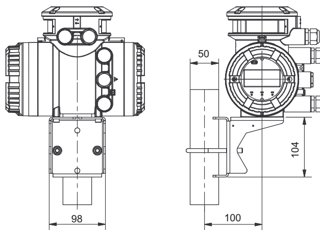
Fig. 21: Dimensions of transmitter in mm, attached to mounting bracket.
